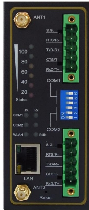
Figure 3.4 Front Panel of SW5502-TB/Sis
