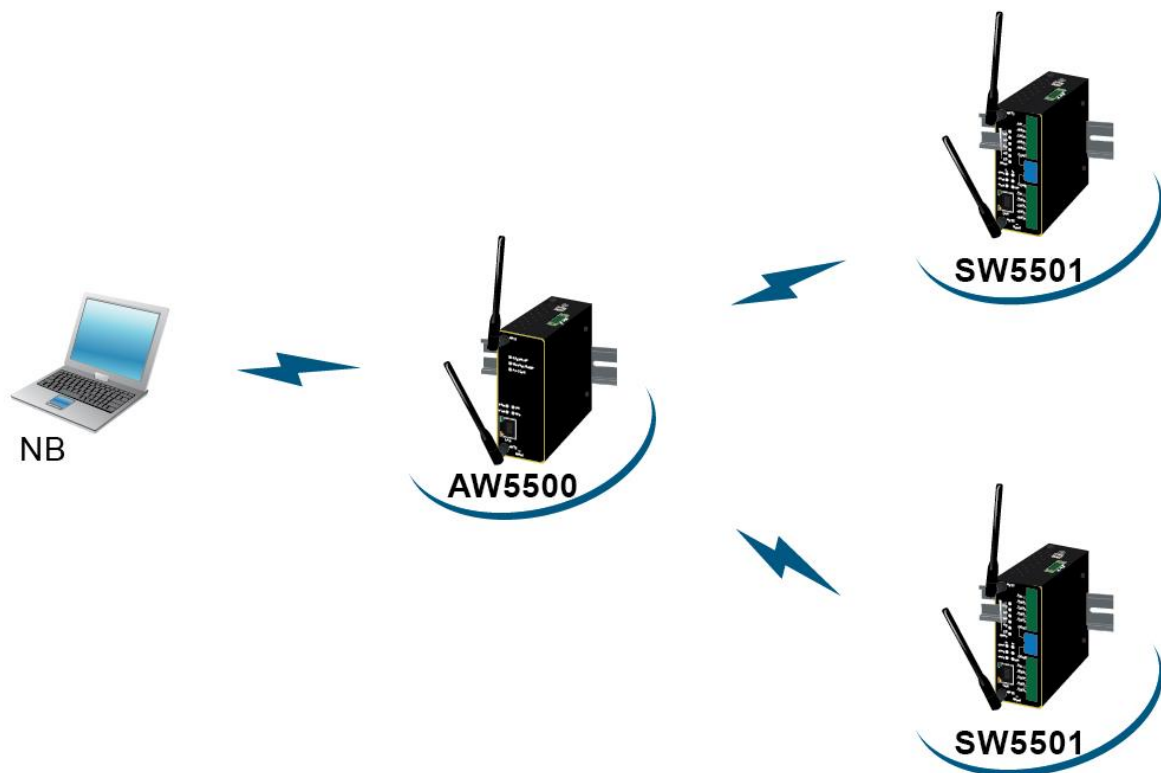
Figure 2.1 An Application of Wireless Serial Device Server in WLAN
