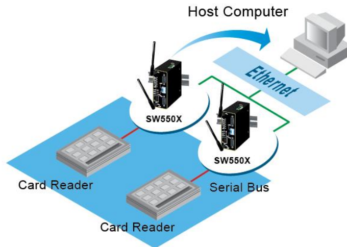
Figure 5.5 An Example of TCP Client Link Mode
