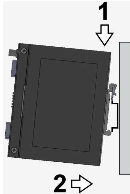
Figure 3.7 Din-Rail Mount of SW550X
